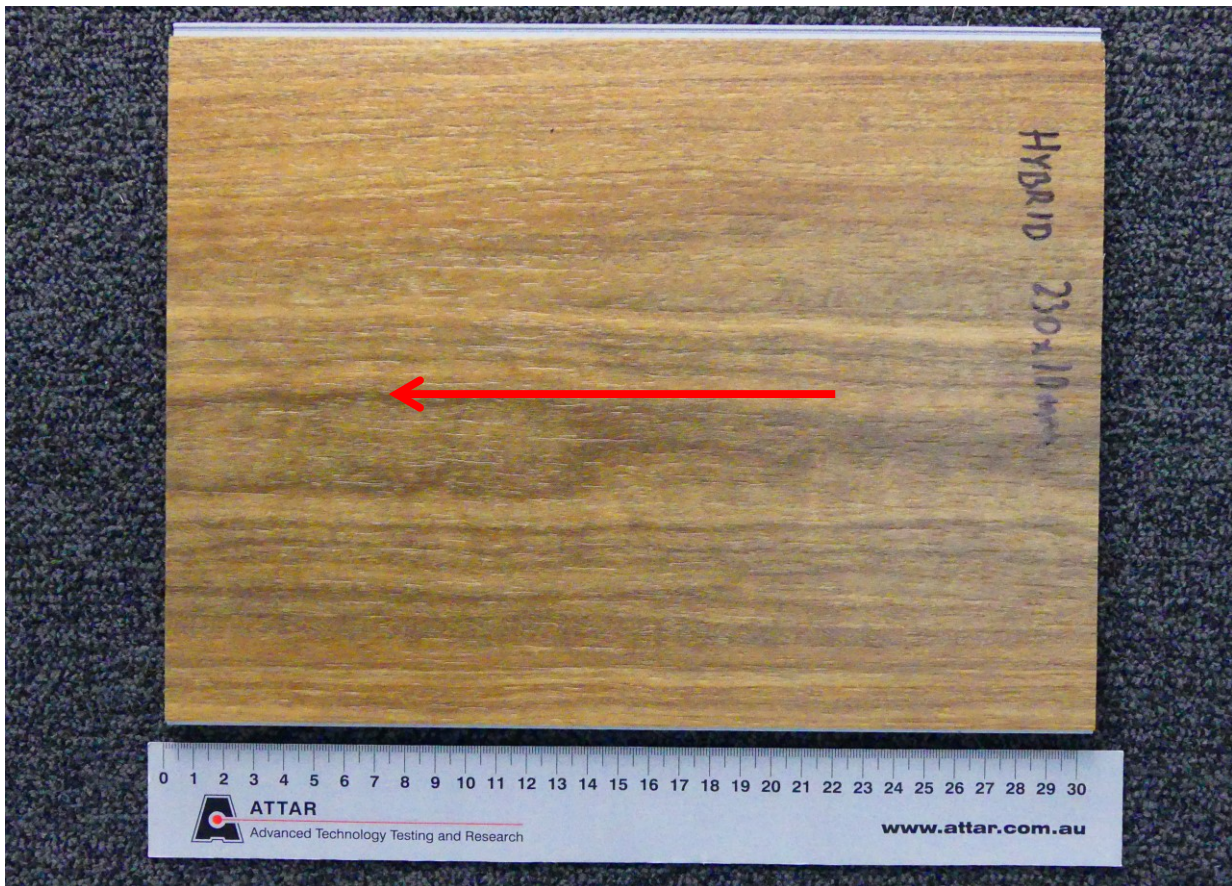
Figure 1: GreenEarth LSPC Hybrid 230x10mm Arrow indicates direction of testing
